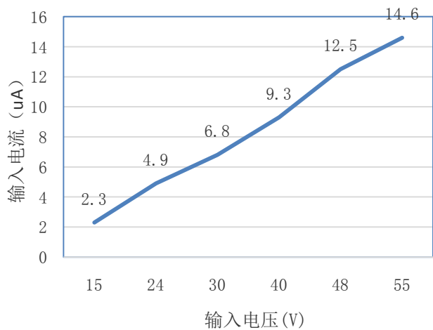
EN关机电流
