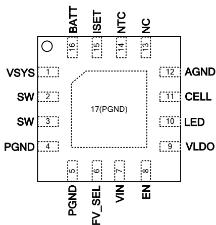
QFN-3X3-16 (Top View)
