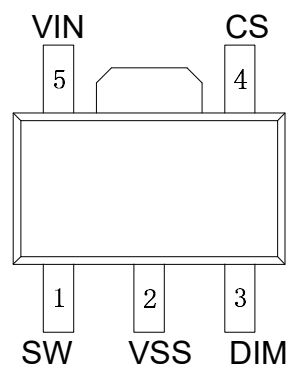
SOT89-5
